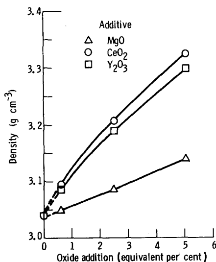
Figure 2 Densities of \text{Si}_3\text{N}_4 with oxide additions after hot pressing at 1750°C and 27.6 MPa (4000 psi) for 30 min.
