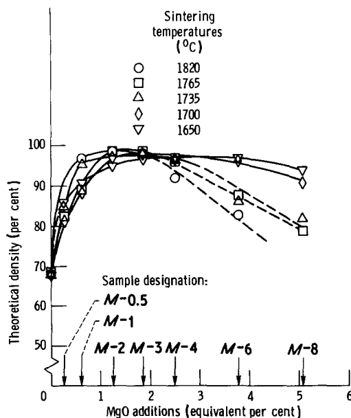
Figure 3 Effect of \text{MgO} additions and sintering temperature on density of pressureless sintered \text{Si}_3\text{N}_4 . (All samples sintered 4 h in \text{N}_2 ).
