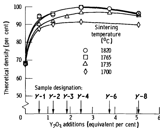
Figure 5 Effect of \text{Y}_2\text{O}_3 additions and sintering temperature on density of pressureless sintered \text{Si}_3\text{N}_4 . (All samples sintered 4 h in \text{N}_2 ).
