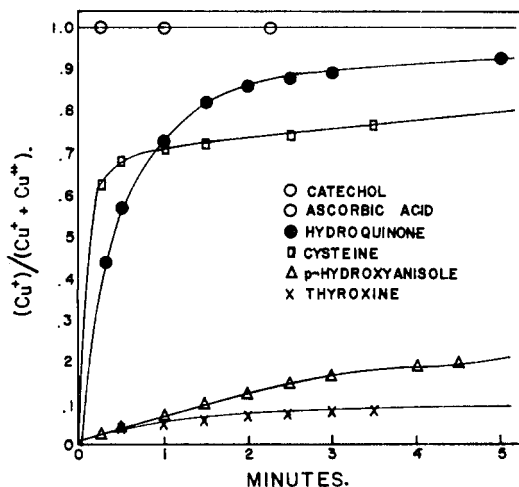
Fig. 2.—Relative rates of cuprous ion formation for several different organic compounds. The formation of the cuprous cuproin complex was measured at 545 m \mu . The reaction was initiated by the addition of the test compound (final concentration 1.00 \times 10^{-4} M ). The reaction mixture contained 0.010 M tris buffer, pH 7.2, 5.00 \times 10^{-6} M \text{Cu}^{\text{II}} , 1.00 \times 10^{-4} M cuproin at 30.0° and 70% acetone.
