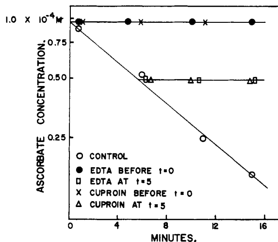
Fig. 1.—Effect of cuproin ( 1.00 \times 10^{-5} M ) and EDTA ( 1.00 \times 10^{-5} M ) added at the indicated times. The reaction mixture consisted of a 50% ethanol-water solution of 5.00 \times 10^{-6} M \text{ Cu}^{\text{II}} , 0.010 M tris buffer, pH 7.2, and 1.00 \times 10^{-4} M ascorbate at 30.0^\circ . Ascorbate concentration was determined in a Beckman spectrophotometer at 265 \mu .
