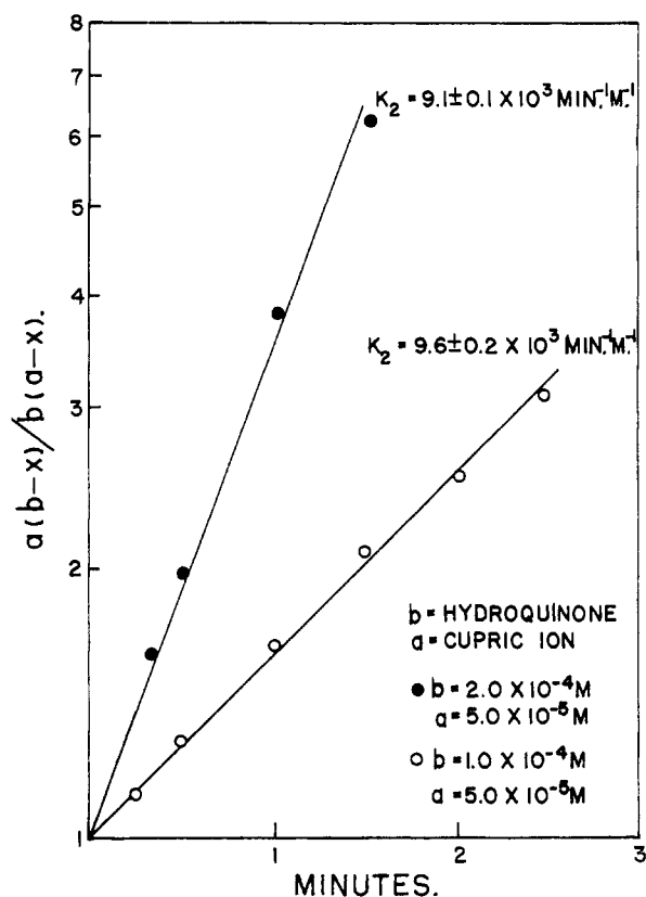
Fig. 3.—Second order plot of the reaction between hydroquinone and cupric ion. Reaction conditions are 30.0°, 0.010 M tris buffer, pH 7.2, cuproin = 2 \times 10^{-4} M in 70% acetone; a and b are the initial concentrations of cupric ion and hydroquinone, respectively, x is the amount of cuprous ion formed at the indicated times. The reaction is followed by measuring the \text{Cu}^{\text{I}} formed by its colored complex with the cuproin reagent at 545 \text{m}\mu .
