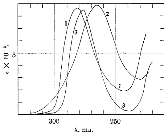
Fig. 2.—Spectrum of the cation of III, obtained by subtraction of the absorption of KI from that of III, (1); spectrum of N-phenylpyridinium chloride (2); spectrum of 3,5-diethyl-2-propylpyridinium ion (3) in 1.2 N HCl in 90% methanol.
