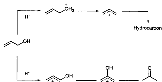
Scheme 1 Reaction scheme for the conversion of allyl alcohol to acetone
