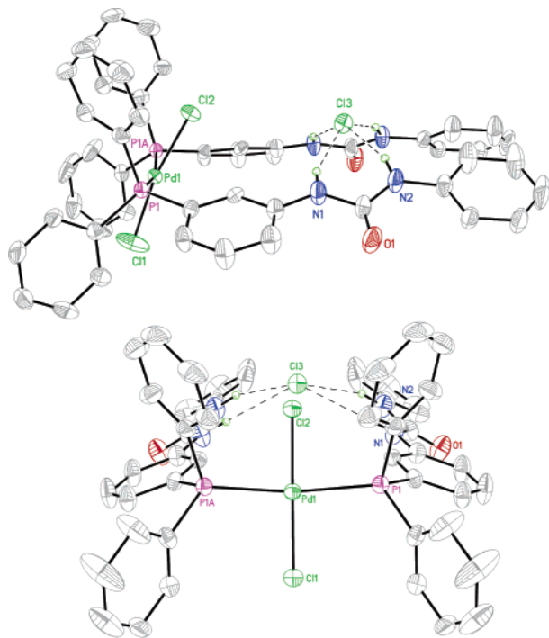
Figure 3. X-ray crystal structure of the anion-bound complex [\text{Bu}_4\text{N}][\text{PdCl}_2(\text{L})_2 \cdot \text{Cl}] ( 1 \cdot \text{Cl} ; 50% displacement ellipsoids). For clarity, the [\text{Bu}_4\text{N}]^+ cation and all hydrogens except those of the urea nitrogens N1 and N2 are omitted. Selected bond lengths (Å) and angles (deg): Pd1–Cl1 2.2857(18), Pd1–Cl2 2.3007(16), Pd1–P1 2.3484(10); Cl1–Pd1–P1 93.88(3), Cl2–Pd1–P1 87.25(3), Cl1–Pd1–Cl2 169.59(8), P1–Pd1–P1A 165.83(5). The suffix A on atom P1A indicates the symmetry operation (x, 1/2 - y, z) .
