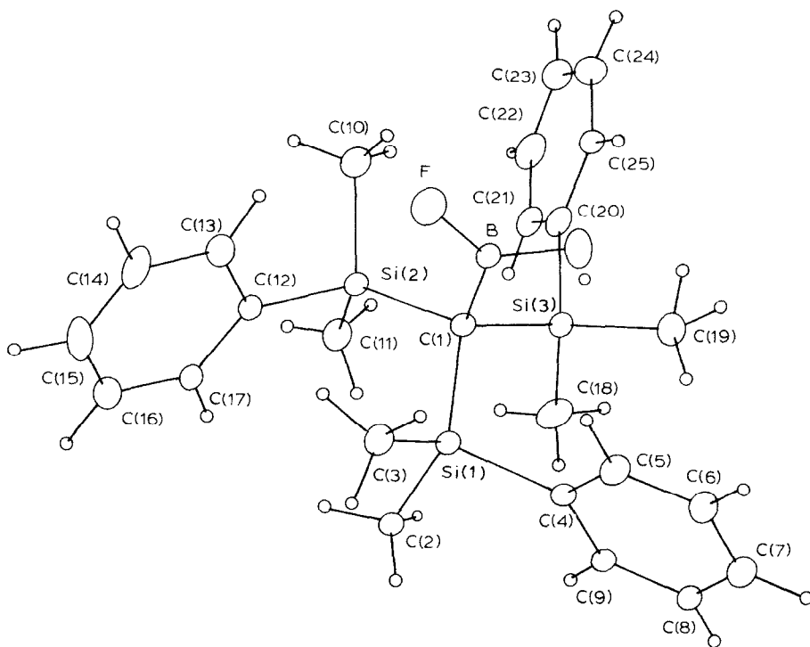
Fig. 1. The structure of (\text{Me}_2\text{PhSi})_3\text{CBF(OH)} .
