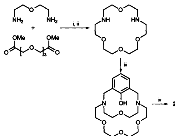
Scheme 1 Synthesis of chromogenic reagent 2 . Reagents and conditions (yields): i, MeOH, room temp., 3 d, reflux 24 h (47%); ii, BH 3 ·SMe 2 in THF (99%); iii, 2,6-bis(bromomethyl)anisole, MeCN, reflux 24 h (75%); iv, p -nitrophenyldiazonium chloride, NaOH, 0 °C (84%).
