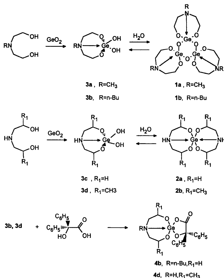
Scheme 1. Cycloaddition of diethanolamine to germanium dioxide.
