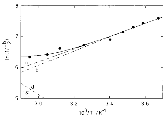
Fig. 2. Effect of temperature on the transverse relaxation rate 1/T_2^b of the e-H 2 O of 2.5 \times 10^{-3} M [\text{Rh}_2(\text{e-H}_2\text{O})_8(\text{a-H}_2\text{O})_2]^{4+} in ^{17}\text{O} enriched water (7.5 at.%) containing 0.1 M \text{Mn}(\text{CF}_3\text{SO}_3)_2 and 1.5 M \text{CF}_3\text{SO}_3\text{H} , and deduced quadrupolar contribution 1/T_{2Q}^b (a: for \Delta S^\ddagger = -60 \text{ J K}^{-1} \text{ mol}^{-1} ; b: for \Delta S^\ddagger = -120 \text{ J K}^{-1} \text{ mol}^{-1} ) and kinetic contribution k (c and d, respectively).
