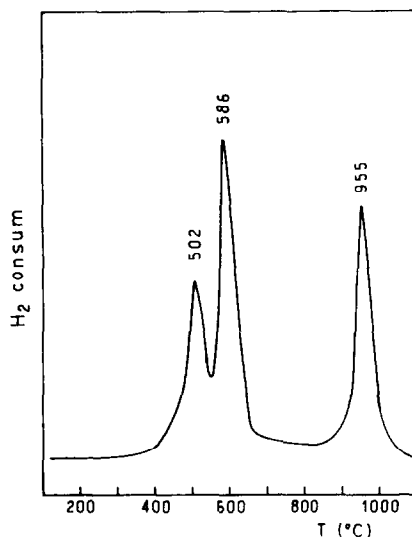
Fig. 1. TPR pattern of the \text{AlVMoO}_7 phase.
