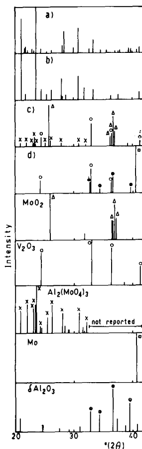
Fig. 3. Comparison of the XRD patterns of: a, \text{AlVMoO}_7 without thermal treatment; b, c, and d, correspond to samples heated at 500, 600 and 1000^\circ\text{C} respectively. Additional patterns are included for reference.
