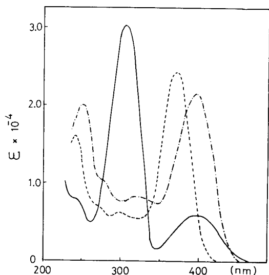
Figure 1. The uv-absorption of the substitution products by amines, 3a (—), 4a (---) and 4c (—•—), in ethanenitrile.
