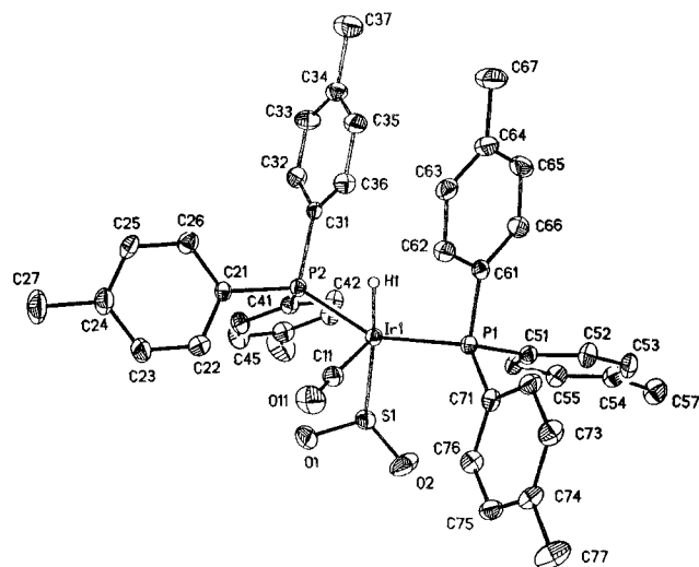
Figure 1. Molecular geometry and labeling of atoms for \text{Ir}(\text{CO})(\text{H})(\text{SO}_2)(\text{P}(p\text{-tolyl})_3)_2 shown by an ORTEP2 diagram with 20% probability contours for the atomic vibration ellipsoids. Hydrogen atoms (other than the hydride ligand, \text{H}(1) ) have been omitted for the sake of clarity.
