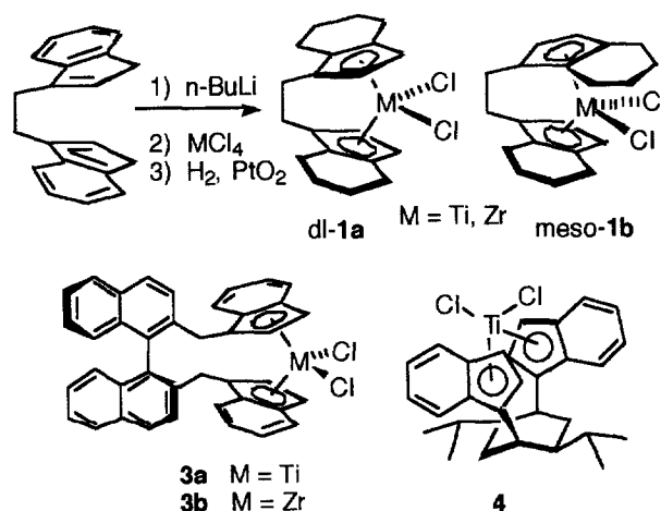
Examples of resolved ansa -metallocenes
