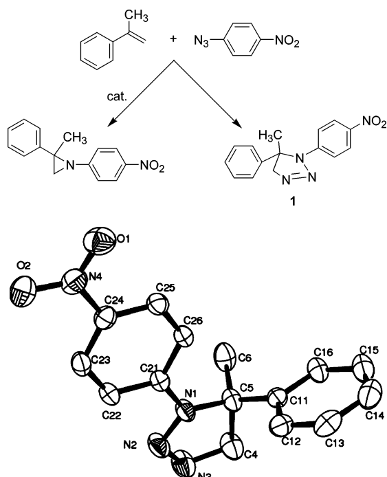
Figure 2. Ortep drawing of 1 . Selected bond lengths (Å): N3–N2 = 1.244(3); N2–N1 = 1.373(2); N1–C5 = 1.483(2); C4–C5 = 1.546(3); C4–N3 = 1.452(3). See the Supporting Information for details.
