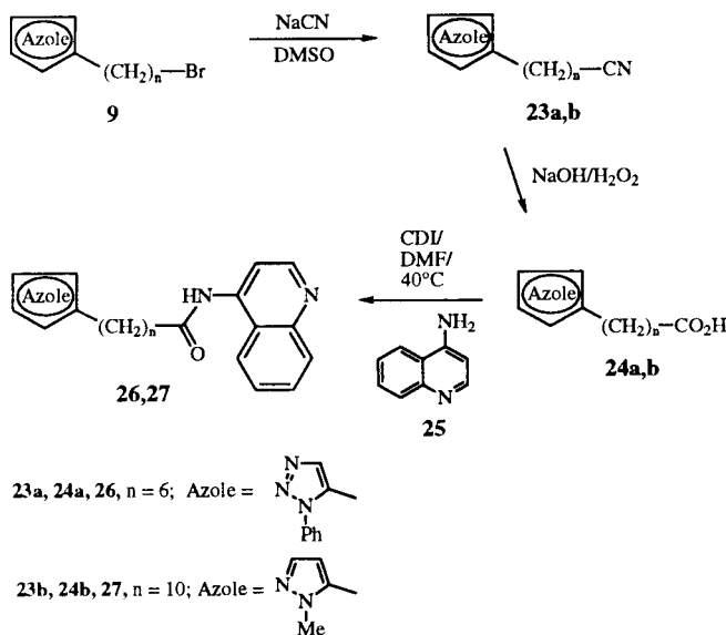
Scheme 5
