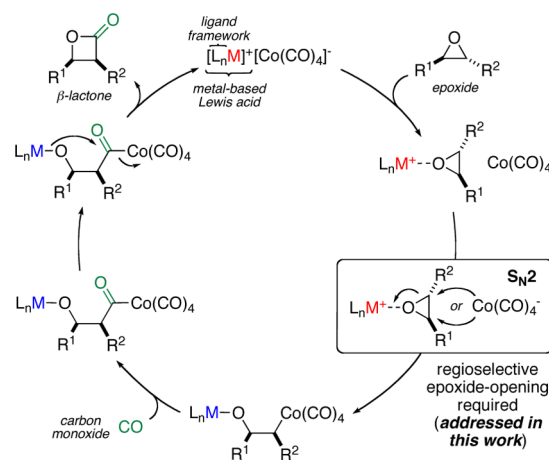
Scheme 2. Simplified Mechanism of Epoxide Carbonylation Using [\text{Lewis Acid}]^+[\text{Co}(\text{CO})_4]^- Catalysts, and the Problem of Regioselectivity
