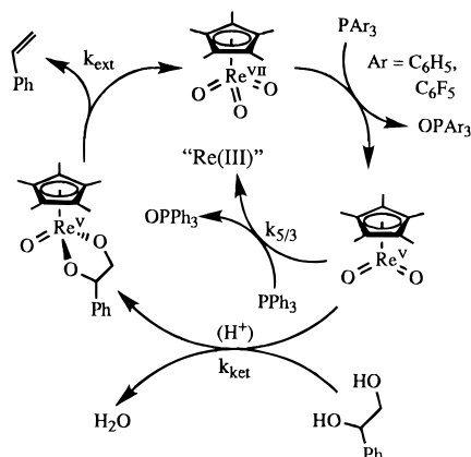
Scheme 1. Catalytic Cycle for Diol Deoxydehydration to Alkenes a
