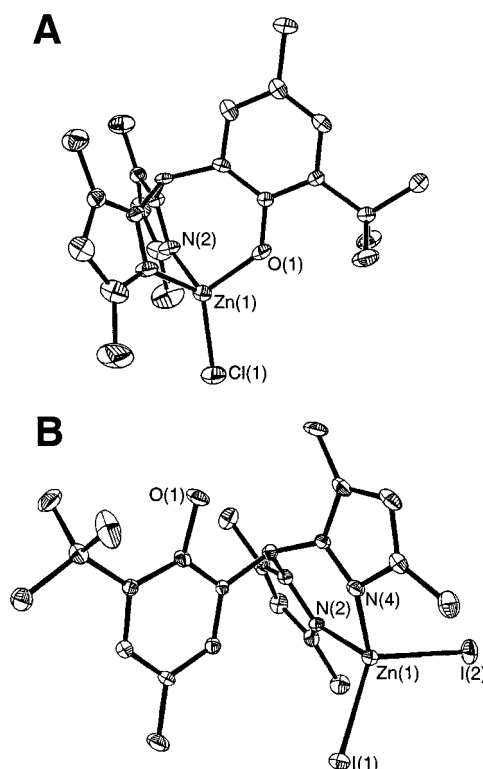
Figure 1. ORTEP diagram with 30% thermal ellipsoids for (a) [(L1O)–ZnCl] and (b) [(L1OH)ZnI 2 ] showing atomic labeling for the coordination sphere only.
