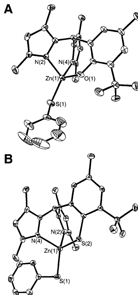
Figure 4. ORTEP diagram with 30% thermal ellipsoids for (a) [(L1O)-ZnSPh] and (b) [(L2S)ZnSPh] showing atomic labeling for the coordination sphere only.
