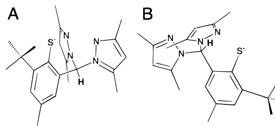
Figure 6. Facial (A) and inverted umbrella (B) configurations of (L2S) – .
