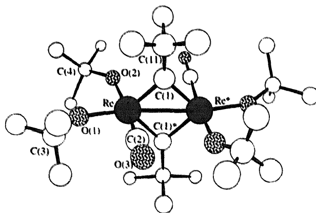
Fig. 2. An ORTEP drawing of the structure of [\text{Re}(\text{O}^t\text{Bu})_2(\text{CO})]_2(\mu\text{-C}^t\text{Bu})_2 .
