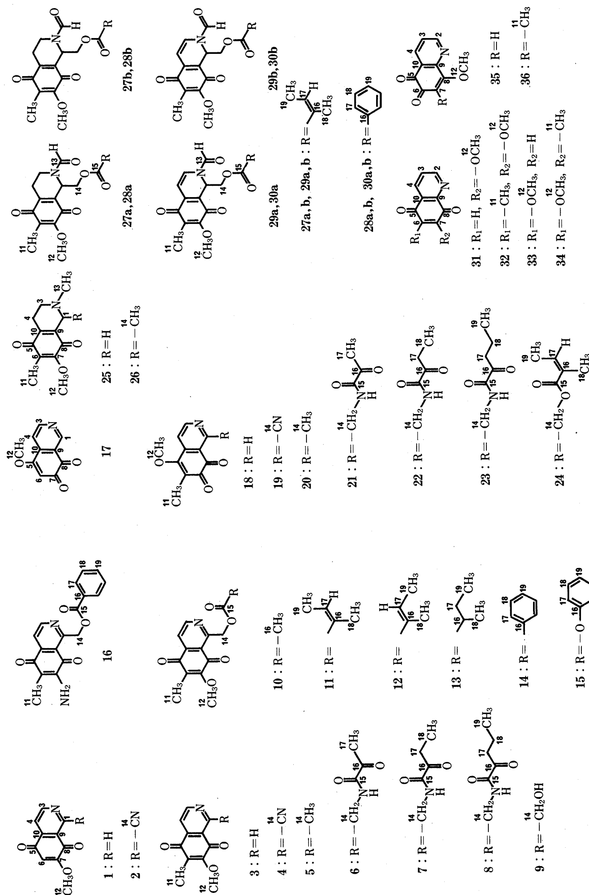
Fig. 1. Isoquinoline and Quinolone Quinones
