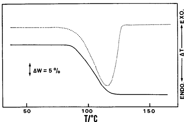
Fig. 1. TG (solid line) and DTA (broken line) curves for the dehydration of \text{Zn}(\text{HCO}_2)_2 \cdot 2\text{H}_2\text{O} in a self-generated atmosphere. Heating rate, 10^\circ \text{C min}^{-1} .
