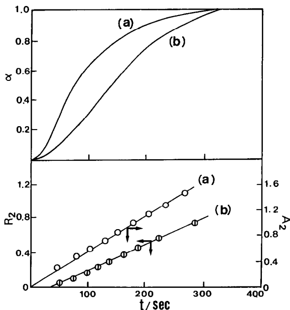
Fig. 2. Typical \alpha vs. t and G(\alpha) vs. t plots for the dehydration of \text{Zn}(\text{HCO}_2)_2 \cdot 2\text{H}_2\text{O} : (a) at 100^\circ\text{C} , 0.12 Torr of water vapour pressure; (b) at 100^\circ\text{C} , 4 Torr of water vapour pressure.
