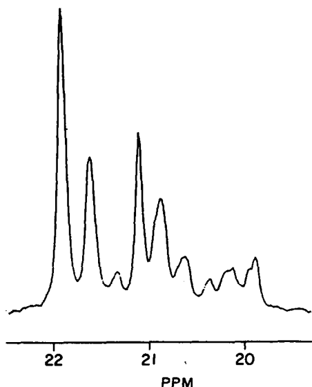
Fig. 2. ^{13}\text{C} NMR methyl pentade signals of the polypropylene obtained at the 6\text{C} /methylalumoxane catalyst at -30^\circ\text{C} .
