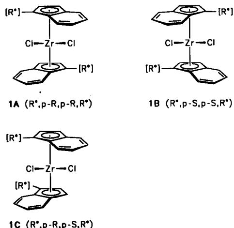
Scheme 1. The three diastereomeric chiral bis( \eta^5 -1- [R^*] -4,5,6,7-tetrahydroindenyl)zirconocenedichlorides ( [R^*] denotes a pair of homochiral substituents per bent metallocene unit; relative configurations of the diastereomers are given in parentheses).
