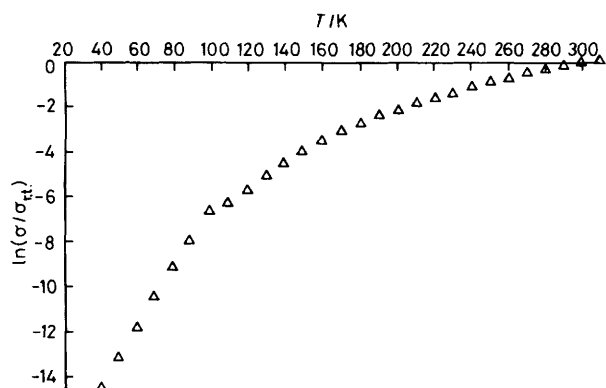
Figure 1. Variation of \ln(\sigma/\sigma_{r.t.}) with temperature for \text{Cu}[\text{Ni}\{\text{S}_2\text{C}_2(\text{CN})_2\}_2] \cdot 2\text{H}_2\text{O}
