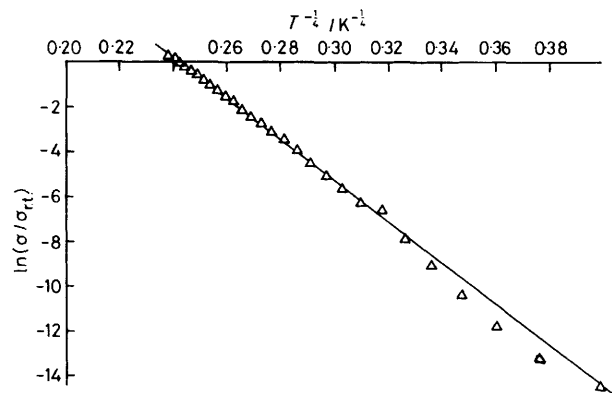
Figure 2. Variation of \ln(\sigma/\sigma_{r.t.}) with T^{-1} for \text{Cu}[\text{Ni}\{\text{S}_2\text{C}_2(\text{CN})_2\}_2] \cdot 2\text{H}_2\text{O}
