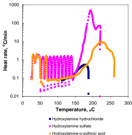
Fig. 5. Heat rate for some hydroxylamine family members. Solid 100% concentration.
