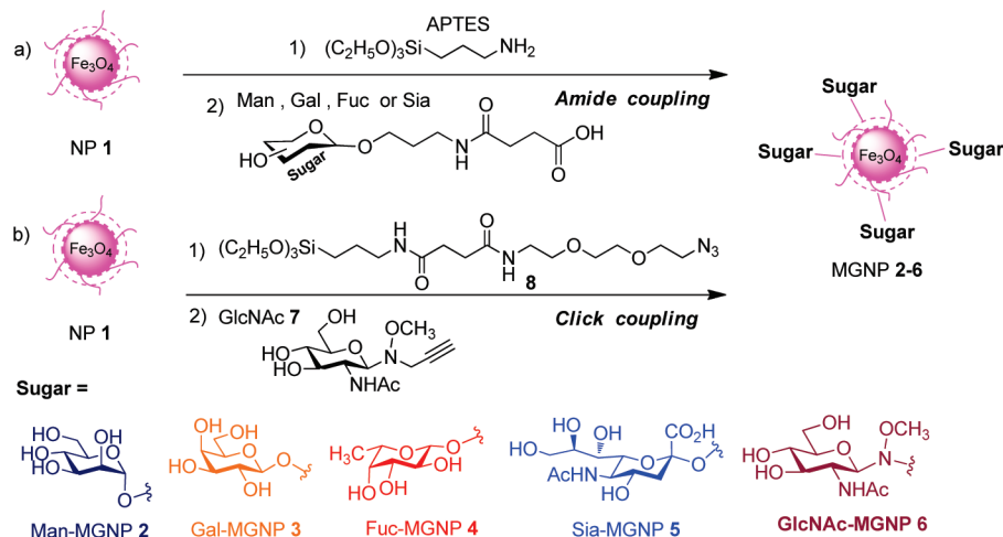
Scheme 1. Synthesis of MGNPs
