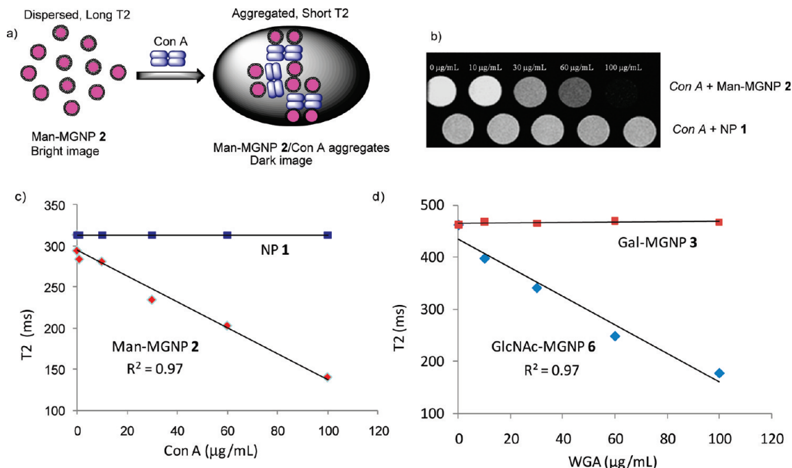
Figure 3. (a) Incubation of Man-MGNP 2 (shown as pink balls) with Con A, a tetrameric mannose selective lectin (shown as blue rectangles) resulted in the formation of aggregates, leading to shorter T_2 relaxation time and consequently a darkened MRI image. (b) T_2 -weighted MRI images of Man-MGNP 2 (20 \mu\text{g/mL} ) and NP 1 (20 \mu\text{g/mL} ) upon incubation with increasing concentrations of Con A. (c) T_2 changed linearly upon incubation of Man-MGNP 2 with increasing concentrations of Con A, while incubation with NP 1 devoid of carbohydrates did not lead to any change. (d) T_2 changed linearly upon incubation of GlcNAc-MGNP 6 with increasing concentrations of the GlcNAc-selective lectin WGA, while incubation with the nonbinding Gal-MGNP 3 did not cause any T_2 change.
