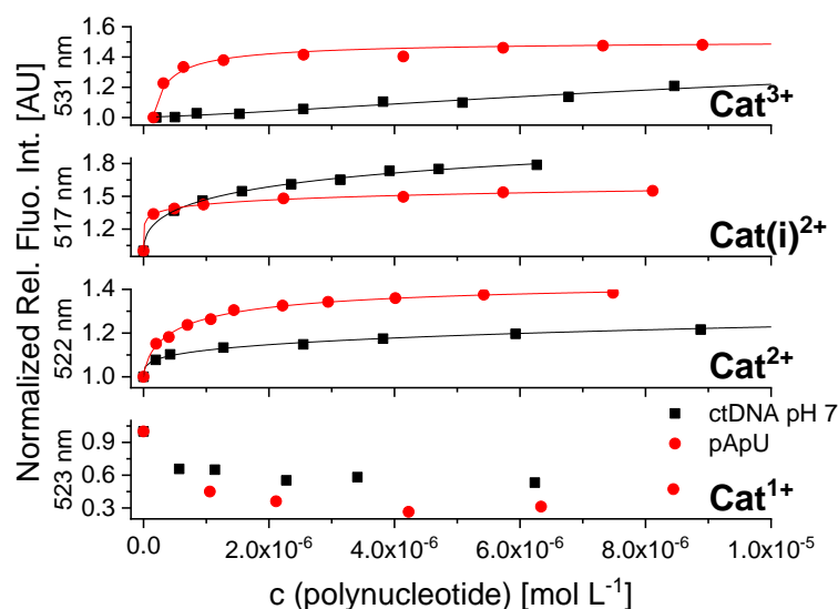
Figure 11: Normalized fluorimetric titration of Cat 1+ ( c = 1 \times 10^{-7} \text{ mol L}^{-1} ; \lambda_{\text{exc}} = 414 \text{ nm} ), Cat 2+ ( c = 1 \times 10^{-7} \text{ mol L}^{-1} ; \lambda_{\text{exc}} = 422 \text{ nm} ), Cat(i) 2+ ( c = 1 \times 10^{-7} \text{ mol L}^{-1} ; \lambda_{\text{exc}} = 417 \text{ nm} ), Cat 3+ ( c = 1 \times 10^{-7} \text{ mol L}^{-1} ; \lambda_{\text{exc}} = 421 \text{ nm} ) with ctDNA and pApU at pH 7.
