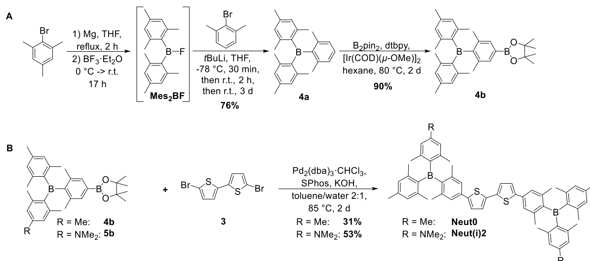
Scheme 1: A) Synthetic route to 4a and 4b . B) Synthetic route to Neut0 and Neut(i)2 .
