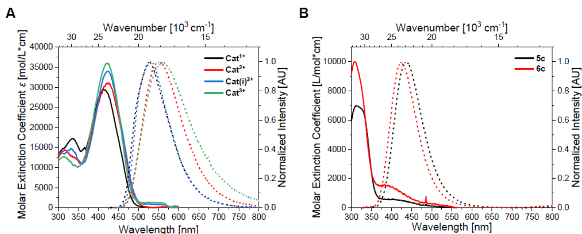
Figure 6: Absorption (solid lines) and emission (dotted lines; excitation at \lambda_{\text{max}}^{\text{abs}} ) spectra of A) the cationic bis -triarylboranes \text{Cat}^{1+} - \text{Cat}^{3+} and B) the cationic triarylboranes 5c and 6c in 1% MeCN in water.
