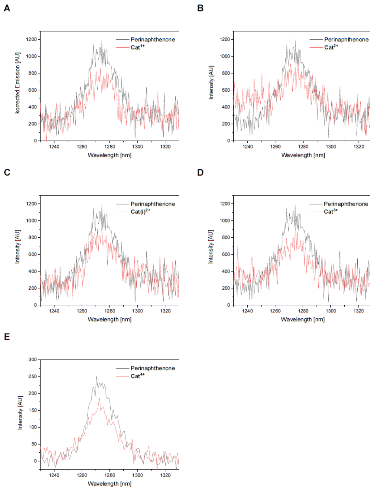
Figure 9: Emission spectra from singlet oxygen sensitization of A) Cat 1+ , B) Cat 2+ , C) Cat(i) 2+ , D) Cat 3+ , and E) Cat 4+ relative to perinaphthenone in acetonitrile.
