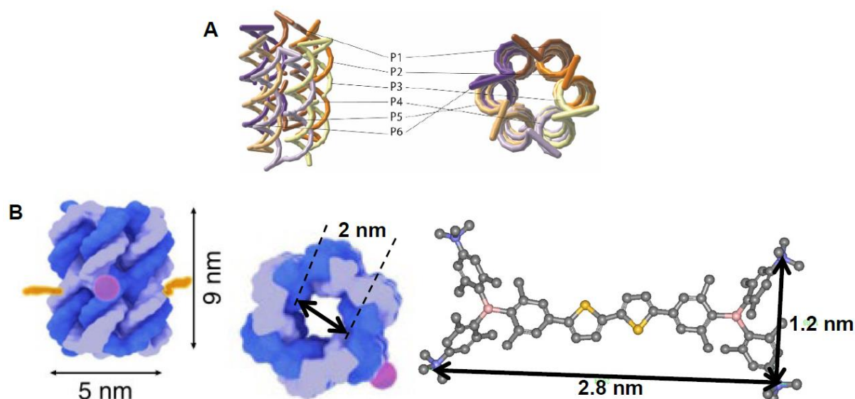
Figure 10: A) Schematic presentation of DNApore. The composition of oligonucleotides P1-P6 is given in Table S21. B) Schematic depiction showing that Cat 4+ and the analogues Cat 1+ -Cat 3+ (width ca. 1.2 nm) fit into the cavity of the DNApore (width ca. 2 nm).
