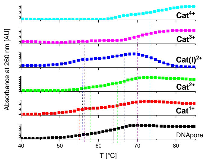
Figure 12: Thermal denaturation curves of DNApore ( c = 2 \times 10^{-5} M at r_{[\text{dye}]/[\text{DNApore}]} = 0.25 ) at pH 8.0 (15 mM Tris-HCl, 300 mM KCl) upon addition of Cat 1+ - Cat 4+ . Error in \Delta T_m values: \pm 0.5 °C.
