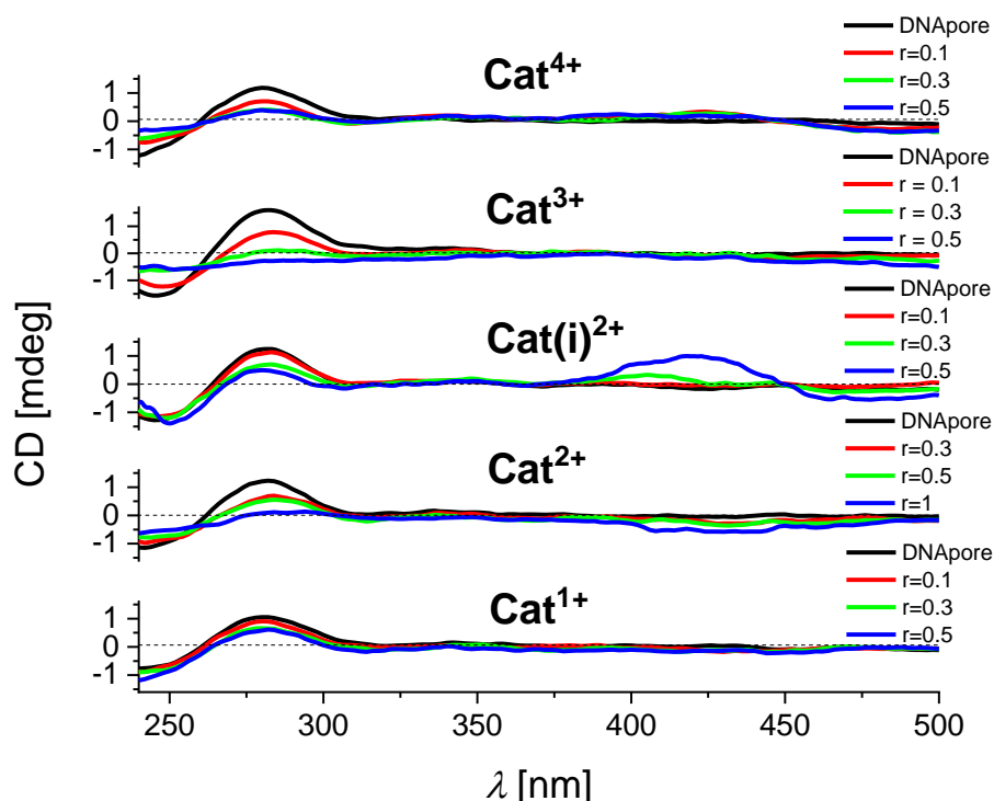
Figure 14: CD titration of DNApore ( c = 5 \times 10^{-5} M) with Cat 1+ - Cat 4+ at molar ratios r_{[\text{dye}]/[\text{polynucleotide}]} = 0.1 - 1 in 15 mM Tris-HCl, 300 mM KCl solutions at pH 8.
