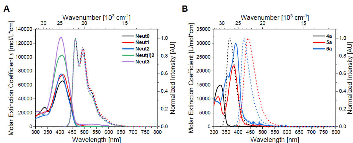
Figure 4: Absorption (solid lines) and emission (dotted lines; excitation at \lambda_{max}^{abs} ) spectra of A) the neutral bis -triarylboranes Neut0-Neut3 and B) the neutral triarylboranes 4a-6a in hexane.
