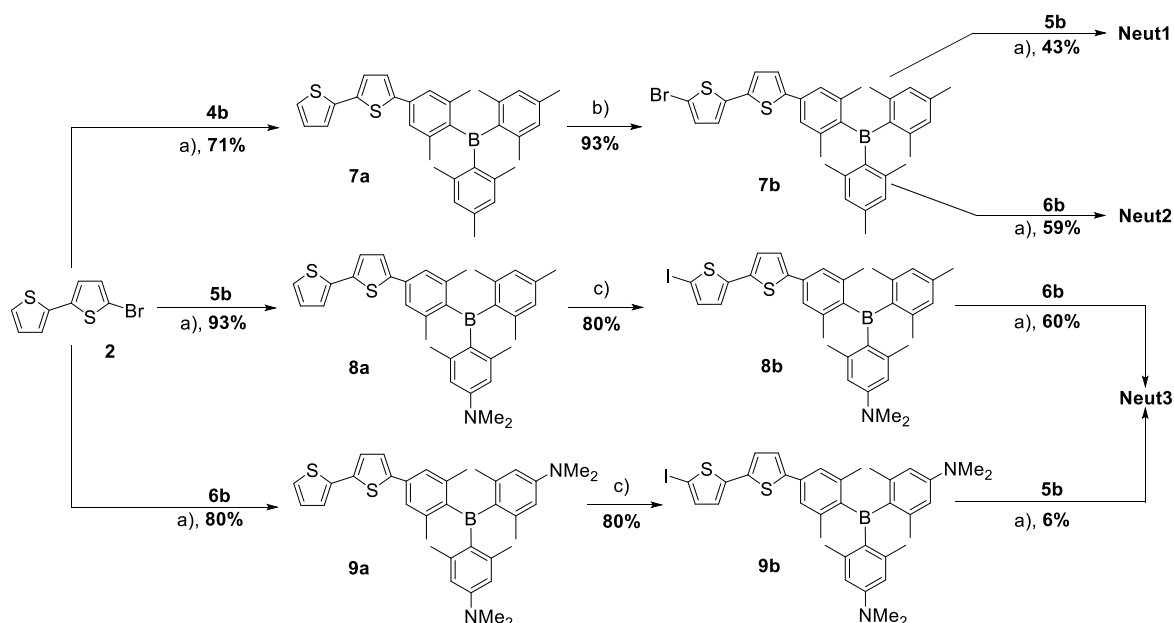
Scheme 2: Synthetic routes to Neut1 , Neut2 , and Neut3 . a) Pd 2 (dba) 3 ·CHCl 3 , SPhos, KOH, toluene/water 2:1, 85 °C, 2 d; b) NBS, DMF, 0 °C, 15 min then r.t., 2 h; c) n BuLi, THF, -78 °C, 1.5 h, then I 2 , -78 °C → r.t., 18 h.
