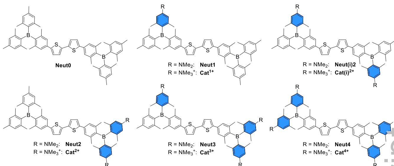
Figure 2: Molecular structures of Neut0-Neut4 and the selectively charged compounds Cat 1+ -Cat 4+ .
