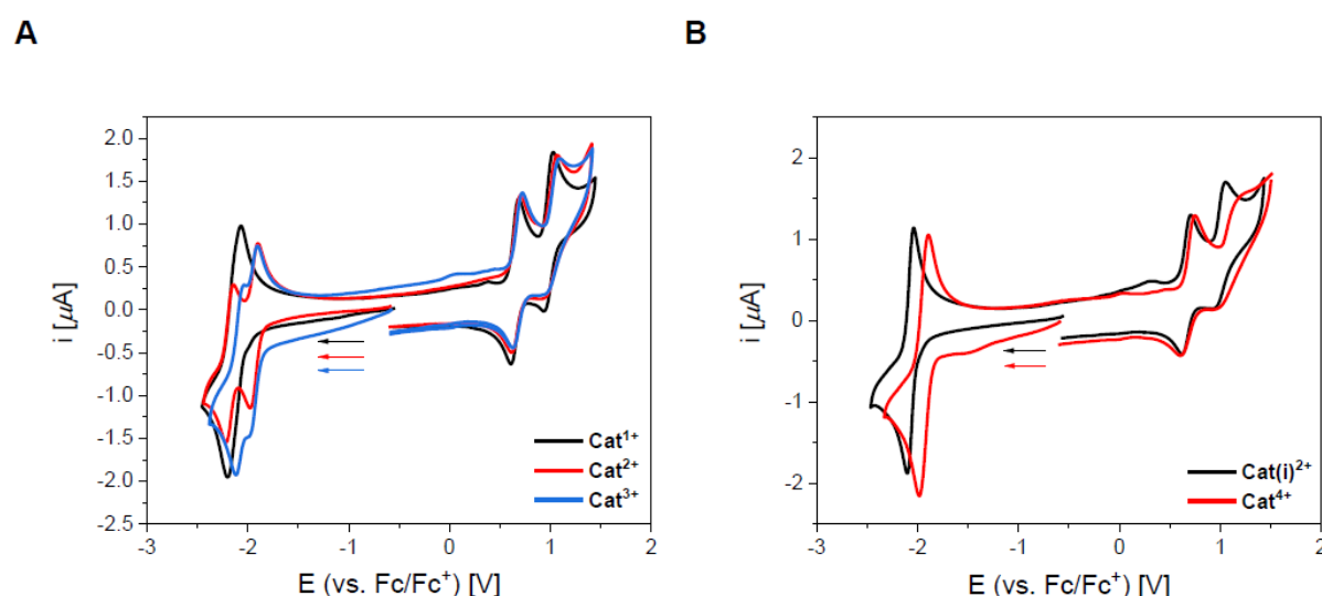
Figure 8: Cyclic voltammograms of Cat1 + -Cat4 + in MeCN.
