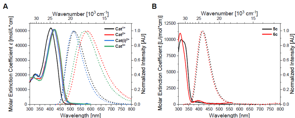
Figure 5: Absorption (solid lines) and emission (dotted lines; excitation at \lambda_{\text{max}}^{\text{abs}} ) spectra of A) the cationic bis -triarylboranes \text{Cat}^{1+} - \text{Cat}^{3+} and B) the cationic triarylboranes 5c and 6c in acetonitrile.
