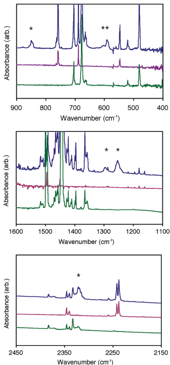
Figure 4. IR spectra showing the absorption bands of \text{C}_6\text{H}_5\text{CN}-\text{BF}_3 in solid argon at 10 K. Bottom traces: \text{BF}_3 in argon, 1:400. Middle traces: \text{C}_6\text{H}_5\text{CN} in solid argon, approximately 1:400. Spectrum was obtained by mixing \text{C}_6\text{H}_5\text{CN} vapor into a stream of pure argon immediately prior to deposition. Top traces: \text{BF}_3 and \text{C}_6\text{H}_5\text{CN} in argon, approximately 1:1:400, obtained by mixing \text{C}_6\text{H}_5\text{CN} vapor into a stream of \text{BF}_3 and argon. Peaks assigned to \text{C}_6\text{H}_5\text{CN}-\text{BF}_3 are marked with asterisks.
