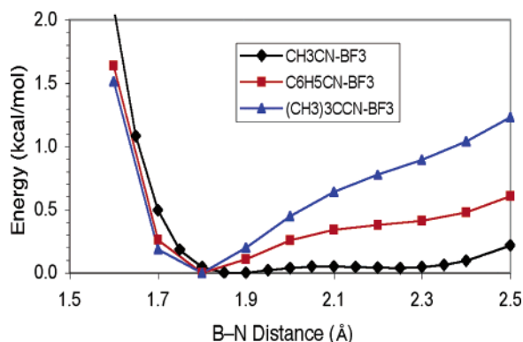
Figure 11. The B–N distance potentials of \text{CH}_3\text{CN}-\text{BF}_3 , \text{C}_6\text{H}_5\text{CN}-\text{BF}_3 , and (\text{CH}_3)_3\text{CCN}-\text{BF}_3 , calculated at the B3LYP/aug-cc-pVTZ ( \text{CH}_3\text{CN}-\text{BF}_3 ) or B3LYP/aug-cc-pV(T|D)Z (others) level of theory.
