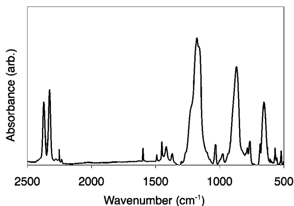
Figure 7. IR spectrum of a bulk solid sample of \text{BF}_3 and \text{C}_6\text{H}_5\text{CN} codeposited at 100 K.
