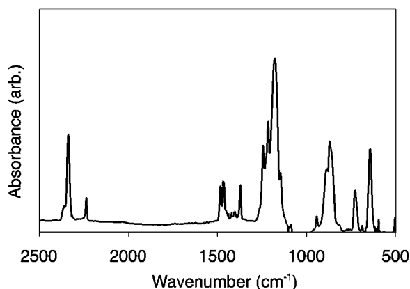
Figure 8. IR spectrum of a bulk solid sample of \text{BF}_3 and (\text{CH}_3)_3\text{CCN} codeposited at 100 K.
