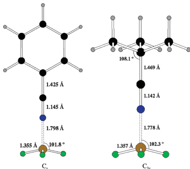
Figure 1. B3LYP/aug-cc-pV(T|D) a Structures of \text{C}_6\text{H}_5\text{CN}-\text{BF}_3 and (\text{CH}_3)_3\text{CCN}-\text{BF}_3 .
