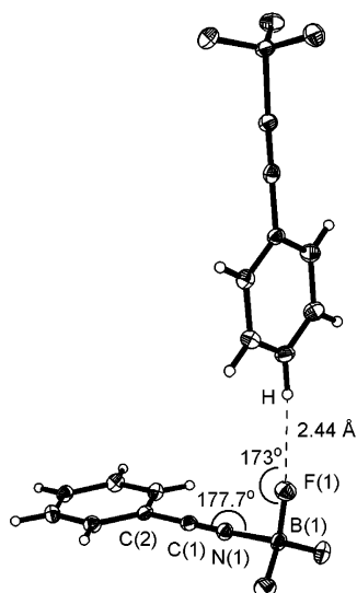
Figure 3. Intermolecular interaction of neighboring \text{C}_6\text{H}_5\text{CN}-\text{BF}_3 complexes in the solid state.
