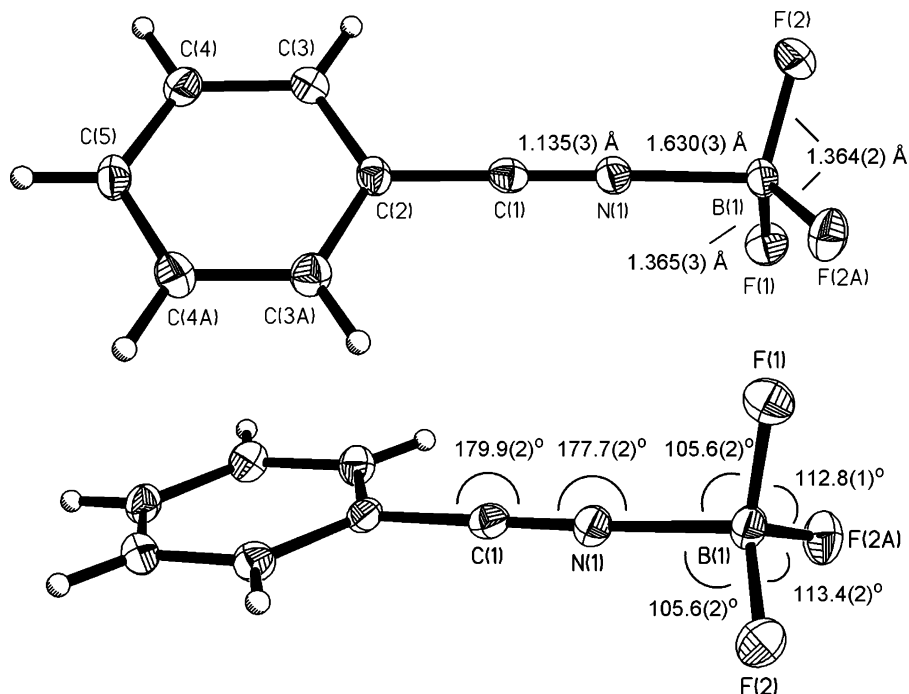
Figure 2. Thermal ellipsoid representations (50% probability boundaries) of the X-ray crystal structure of \text{C}_6\text{H}_5\text{CN}-\text{BF}_3 , with significant interatomic distances (top) and angles (bottom) noted. Atom pairs F(2)-F(2A), C(3)-C(3A), and C(4)-C(4A) are related by a crystallographic mirror plane.
