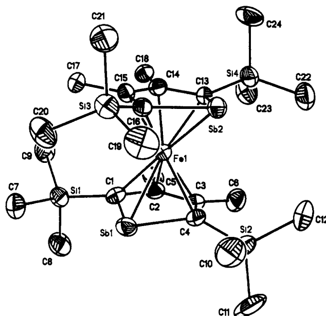
Figure 1. ORTEP drawing of the solid-state structure of 2,2',5,5'-tetrakis(trimethylsilyl)-3,3',4,4'-tetramethyl-1,1'-distibiferrocene (2), with thermal ellipsoids at the 50% probability level.
