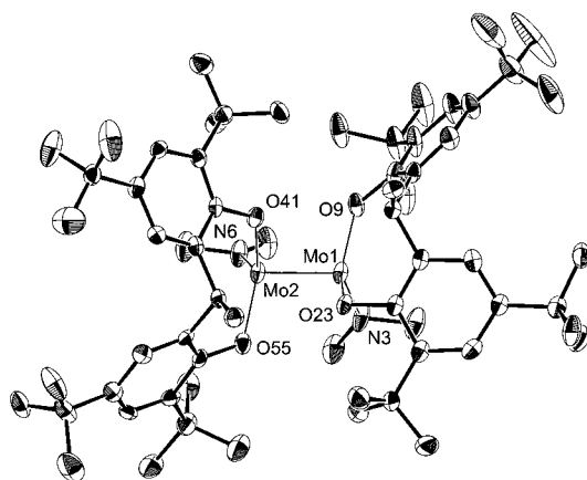
Figure 3. View of the molecular structure (50% thermal ellipsoid probability) of C showing the roof shape of the O~CHMe~O ligand directed away from the Mo-Mo bond.
