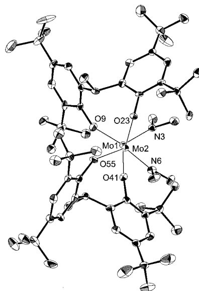
Figure 1. View of the molecular structure (50% thermal ellipsoid probability) of A showing the gauche conformation of the central O_2-NMo\equiv MoNO_2 core.
