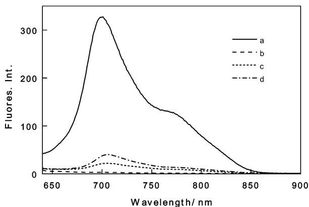
Figure 3. Steady-state fluorescence of (a) C 60 -reference (0.1 mM), (b) C 60 - ortho -TTF (0.1 mM), (c) C 60 - meta -TTF (0.1 mM), and (d) C 60 - para -TTF (0.1 mM) in toluene. \lambda_{\text{ex}} = 520 nm.
