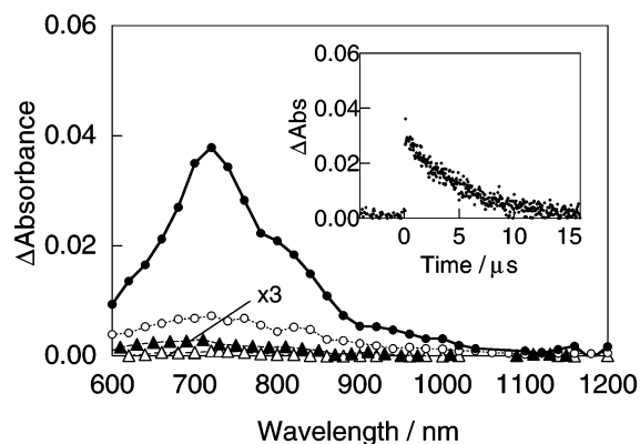
Figure 6. Nanosecond transient absorption spectra of C 60 -reference in benzonitrile after pulse irradiation using 532-nm light: (●) C 60 -reference, (○) C 60 – para -TTF, (▲) C 60 – meta -TTF, and (Δ) C 60 – ortho -TTF. Inset shows a time profile at 720 nm of C 60 -reference.
