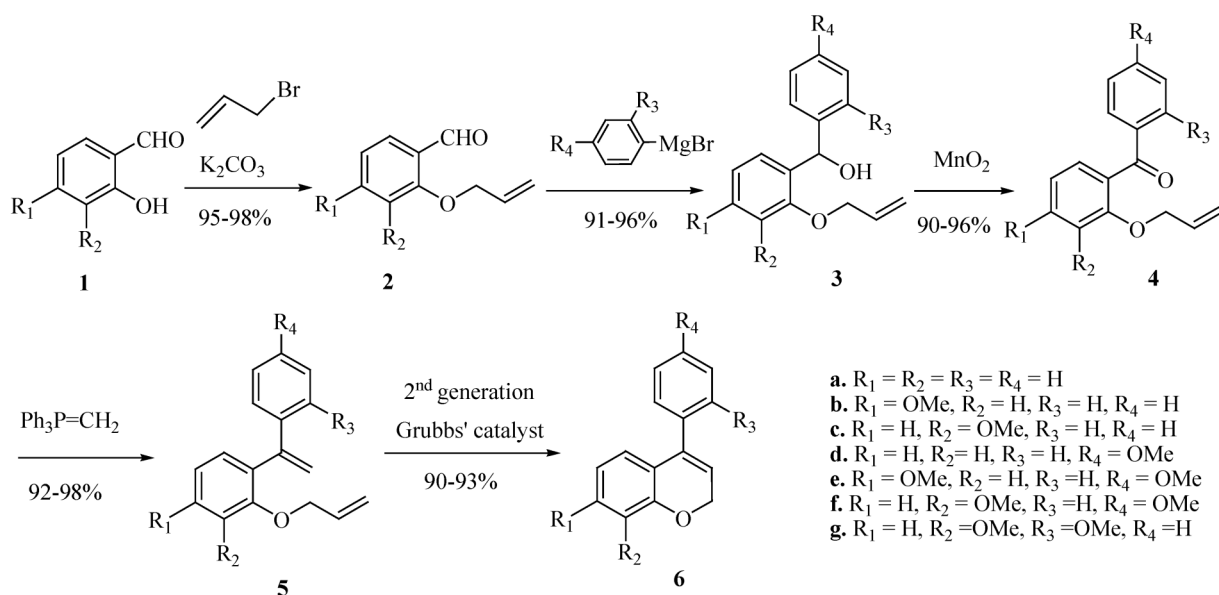
Scheme 1 Synthetic strategy of neoflavenes from salicylaldehydes
