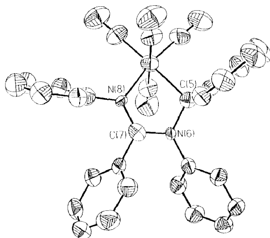
Fig. 1. Molecular structure of (\text{CO})_4\text{Mn}\overline{\text{C}(\text{H})(\text{Ph})\text{N}(\text{Ph})\text{C}=\text{N}(\text{Ph})} . (I)
