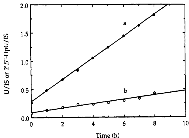
Figure 2. A typical kinetic run, with [morpholine buffer] total = 0.2 M, and B/BH + = 8/2; curve a, uridine (U); curve b, 2',5''-UpU; IS, internal standard.
