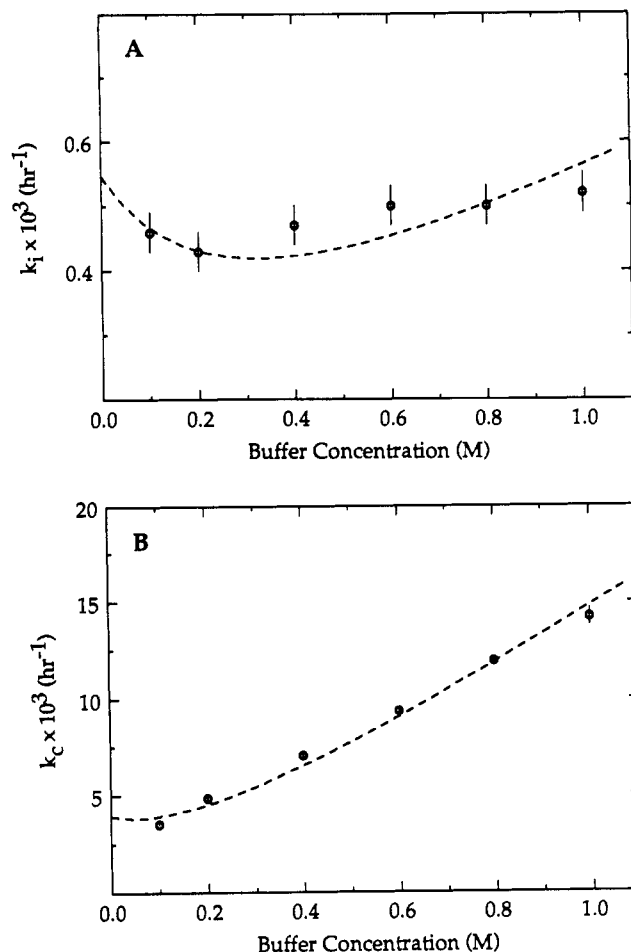
Figure 5. Pseudo-first-order rate constants as a function of buffer concentration for (A) isomerization of 3',5''-UpU and (B) the simultaneous cleavage with 8/2 morpholine/morpholine-HCl. The dashed curves in both parts were derived by fitting the points to eqs 5 and 6 using the same method as in Figure 3, but carrying over from Figure 3 all values that are unaffected by the buffer ratio and pH. The values of the parameters from this curve fitting are listed in Table V.
