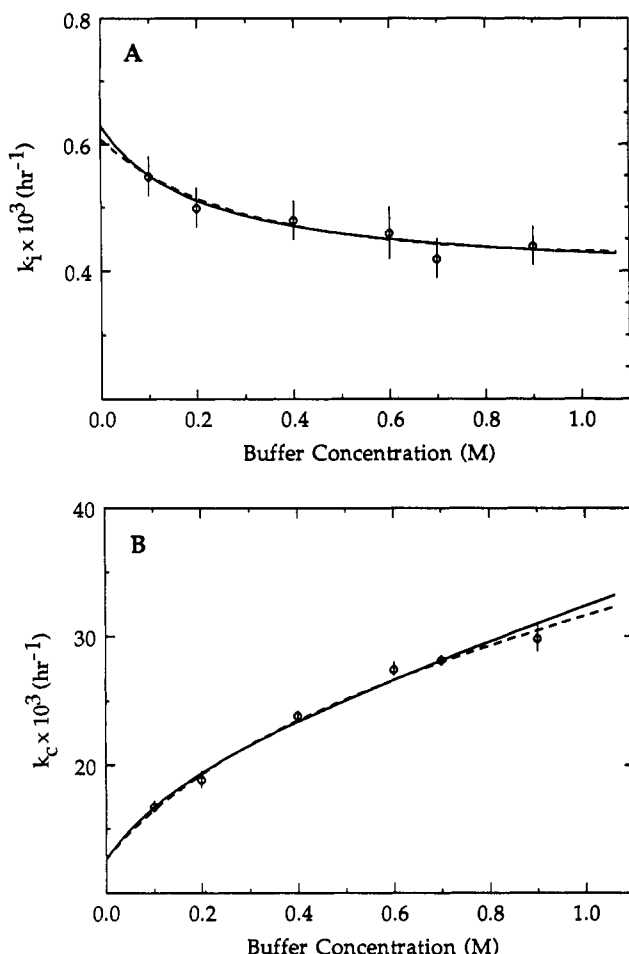
Figure 4. Pseudo-first-order rate constants as a function of buffer concentration for (A) isomerization of 3',5''-UpU and (B) the simultaneous cleavage with 9.5/0.5 morpholine/morpholine-HCl. The solid lines are derived by fitting eqs 3 and 4, while the dashed lines are from fitting eqs 5 and 6. The values of the parameters from this curve fitting are listed in Tables IV and V.
