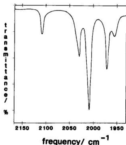
Fig. 2. Infrared spectrum of \text{Re}(\text{CO})_4[\text{P}(\text{OMe})_3]\text{I} recorded in hexane.
