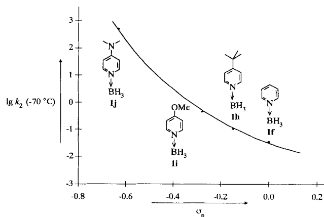
Figure 2. Plot of \lg k_2 (−70 °C, \text{CH}_2\text{Cl}_2 ) for the reaction of pyridine boranes 1f , 1h , 1i , and 1j with 2a versus \sigma_p .
