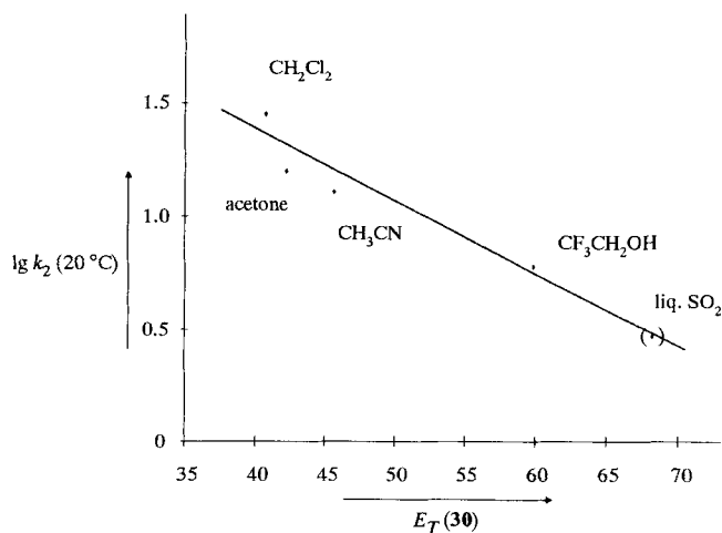
Figure 1. Plot of \lg k_2 (20 °C) for the reaction of 1a with 2a versus Reichardt's E_T(30) values [ \lg k_2 (20 °C) = -3.082 \times 10^{-2} \times E_T(30) + 2.583 , r = 0.976 ]. The rate constant for liquid \text{SO}_2 [ k_2(20^\circ\text{C}) = 2.92 \text{ L mol}^{-1} \text{ s}^{-1} ] was estimated from the relative rate of the reaction of 2d with 1a in \text{SO}_2 and dichloromethane.
