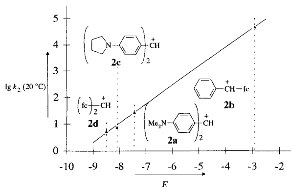
Figure 4. Correlation of the second-order rate constants ( \log k_2 , 20^\circ\text{C} , \text{CH}_2\text{Cl}_2 ) for the reactions of triethylamine borane ( 1a ) with carbocations 2a–d , with their electrophilicity parameters E .
