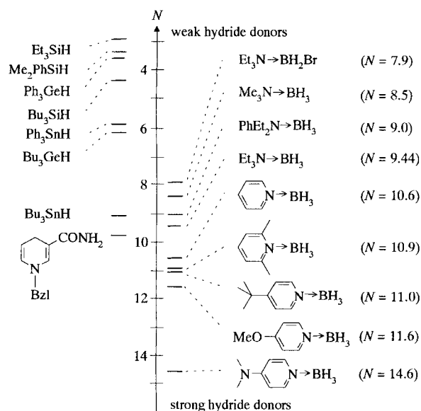
Figure 5. Nucleophilicity N of amine boranes 1 compared with other non-ionic hydride donors.
