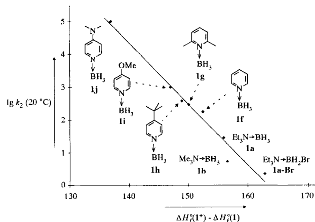
Figure 3. Correlation between the kinetics [ \log k_2(20^\circ\text{C}, \text{CH}_2\text{Cl}_2) ] and the thermodynamics [ \Delta H_f^\circ(1^*) - \Delta H_f^\circ(1) ] of the reaction of 1a–j with 2a ; \log k_2(20^\circ\text{C}) = -0.186(\Delta H_f^\circ(1^*) - \Delta H_f^\circ(1)) + 30.4 , r = -0.987 .
