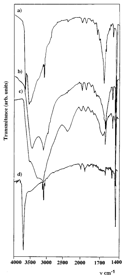
Figure 8. IR spectra for (a) \text{Al}_2(\text{O}_3\text{PC}_6\text{H}_5)_3 \cdot 2\text{H}_2\text{O} , (b) \alpha\text{-Al}(\text{HO}_3\text{-PC}_6\text{H}_5)(\text{O}_3\text{PC}_6\text{H}_5) \cdot \text{H}_2\text{O} , (c) \text{Al}(\text{HO}_3\text{PC}_6\text{H}_5)_3 \cdot \text{H}_2\text{O} , and (d) \text{Al(OH)(O}_3\text{PC}_6\text{H}_5\text{)} .
