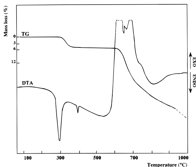
Figure 7. TGA–DTA curves for \text{Al(OH)(O}_3\text{PC}_6\text{H}_5\text{)} .
