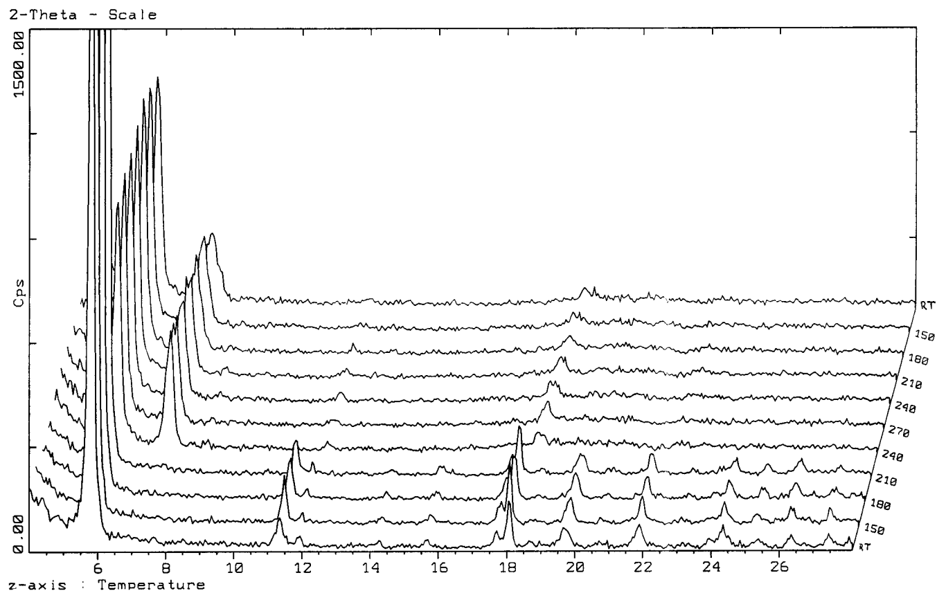
Figure 6. X-ray thermodiffractometric powder patterns for \text{Al}(\text{HO}_3\text{PC}_6\text{H}_5)_3 \cdot \text{H}_2\text{O} .
