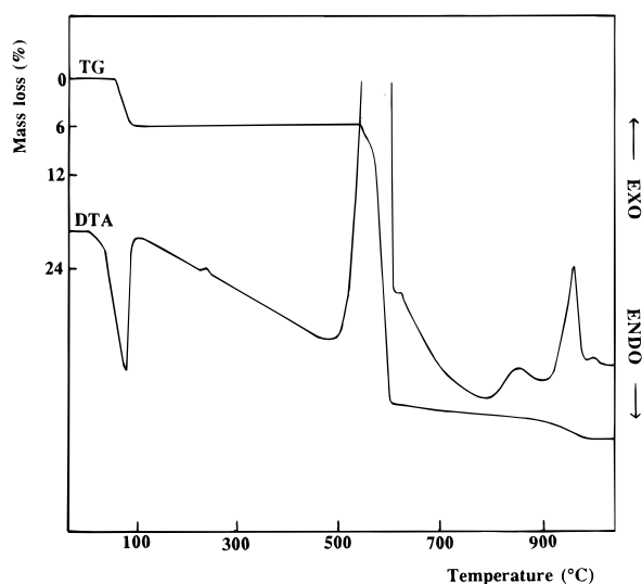
Figure 1. TGA-DTA curves for \text{Al}_2(\text{O}_3\text{PC}_6\text{H}_5)_3 \cdot 2\text{H}_2\text{O} .
