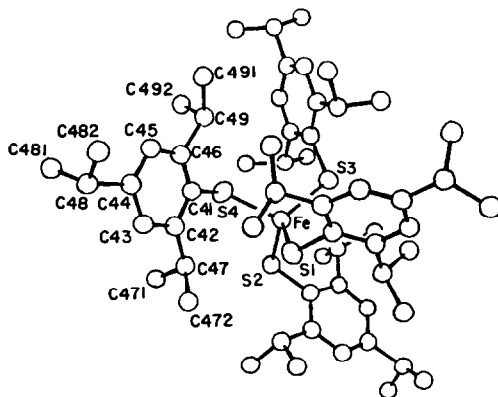
Fig. 1. ORTEP diagram of the anion of [\text{Ph}_4\text{P}][\text{Fe}(\text{SC}_{15}\text{H}_{23})_4] ; selected distances ( \text{\AA} ) and angles ( ^\circ ): Fe–S1 2.263(3) , Fe–S2 2.263(3) , Fe–S3 2.310(3) , Fe–S4 2.252(3) , S1–Fe–S2 106.9(1) , S1–Fe–S3 114.2(1) , S1–Fe–S4 112.4(1) , S2–Fe–S3 112.5(1) , S2–Fe–S4 97.8(1) , S3–Fe–S4 111.7(1) .
