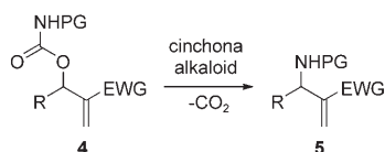
Scheme 4. [1,3]-Sigmatropic decarboxylative rearrangement.
