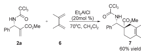
Scheme 3. Diels–Alder reaction between amide product ( 2a ) and 2,3-dimethylbuta-1,3-diene 6 .
