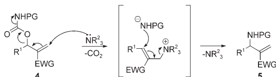
Scheme 5. The domino \text{S}_{\text{N}}2'-\text{S}_{\text{N}}2' mechanism for the decarboxylating rearrangement reaction of carbamate 4 .
