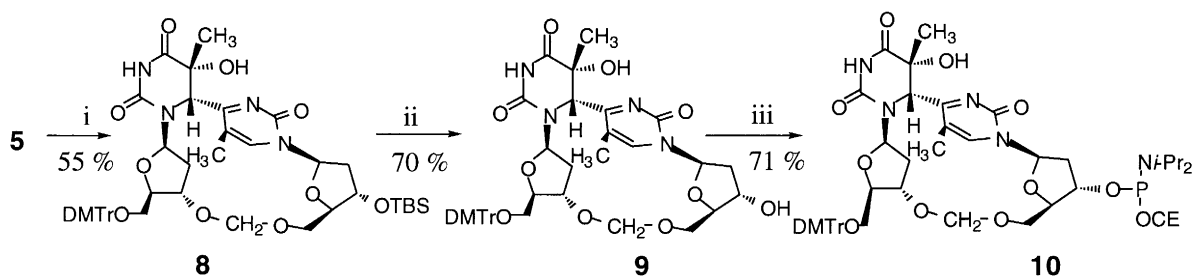
Scheme 2. (i) DMTrCl, pyridine; (ii) TBAF, THF; (iii) i -Pr 2 NP(OCE)Cl, i -Pr 2 NEt, CH 2 Cl 2
