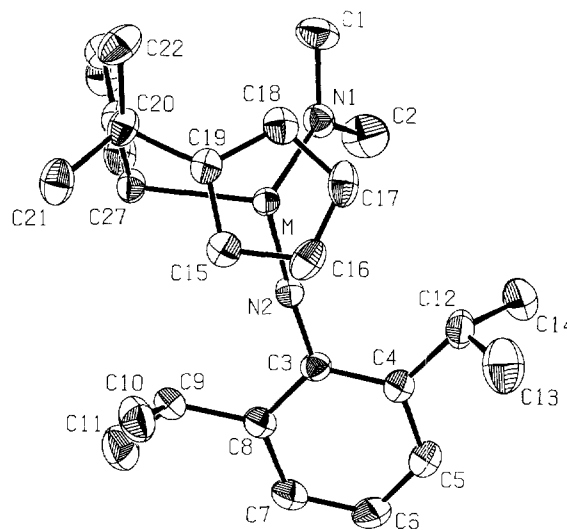
Fig. 3. Structural presentation of the \eta^5:\eta^1 ansa -metalloenes 4a,b perpendicular to the plane of the \eta^5 -coordinated cyclopentadienyl ring. Ellipsoids are drawn at the 50% probability level. Hydrogen atoms are omitted for clarity.
