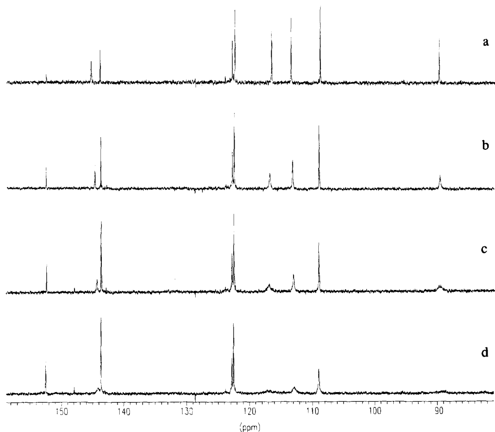
Fig. 6. Variable-temperature ^{13}\text{C} NMR spectra of the \eta^5:\eta^1 ansa -metallocene 4b in the phenyl and cyclopentadienyl range ( \text{thf-d}_8 ): (a) 20 °C; (b) –50 °C; (c) –80 °C; (d) –105 °C.
