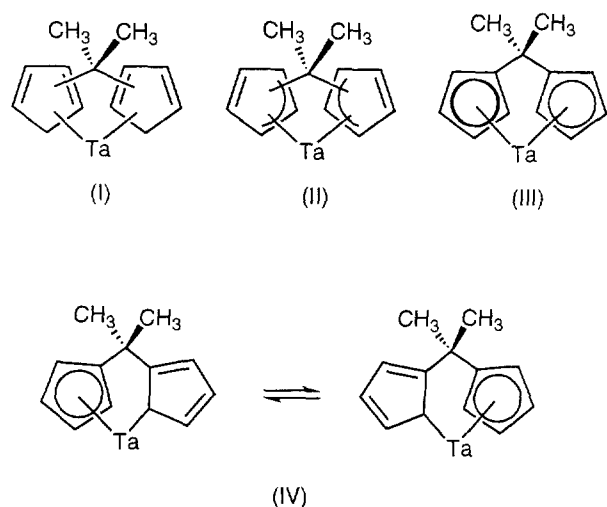
Fig. 4. Conceivable coordination modes for the 2,2-bis(cyclopentadienyl)propane ligand of 4b .
