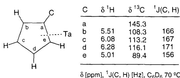
Fig. 5. ^1\text{H} – ^{13}\text{C} NMR chemical shifts and ^1J(\text{C}, \text{H}) coupling constants for the cyclopentadienyl ring of 4b .
