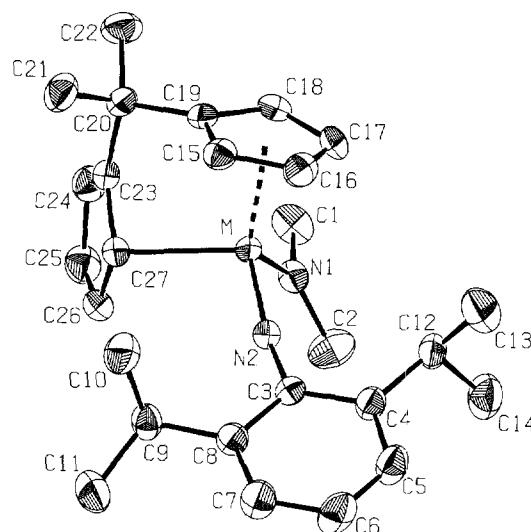
Fig. 2. ORTEP drawing of the crystal and molecular structure of the \eta^5:\eta^1 ansa -metalloenes 4a (niobium) and 4b (tantalum). Ellipsoids are drawn at the 50% probability level. Hydrogen atoms are omitted for clarity.
