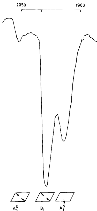
Figure 2. Infrared spectrum of trans -( \text{PnBut}_2\text{Cl} ) _2\text{BrMn(CO)}_3 in the presence of excess \text{PnBut}_2\text{Cl} , in chloroform.
