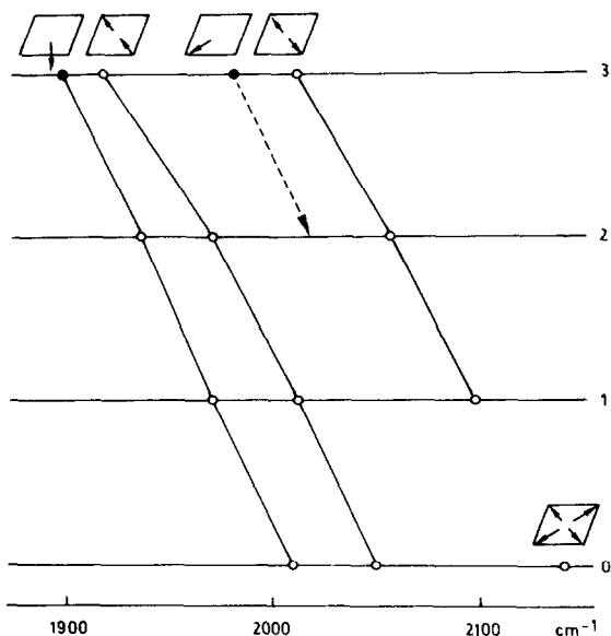
Figure 1. Correlation chart for the CO spectra of \text{Mn(CO)}_{5-n}\{\text{P(OMe)}_3\}_n\text{Br} ; for n = 1 the phosphite ligand stands cis to Br; for n = 2 the trans -isomer is considered; n = 3 : (●) has all the three phosphite ligands cis to Br, (○) has one \text{P(OMe)}_3 group trans to Br and both the other phosphites cis to Br but trans to each other.
