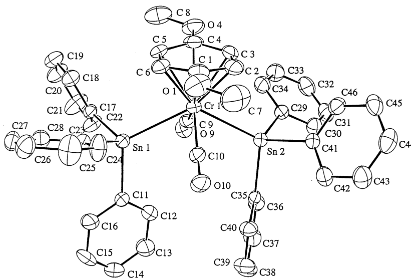
Fig. 2. ORTEP drawing of (\eta^6\text{-}1,4\text{-C}_6\text{H}_4(\text{OCH}_3)_2)\text{Cr}(\text{CO})_2(\text{SnPh}_3)_2 , 3b .
