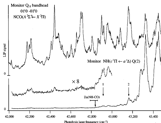
FIG. 5. NCO( X^2\Pi ) and NH( a^1\Delta ) photofragment yield spectra near D_0(\text{NH}+\text{CO}) . Top trace: NCO( X^2\Pi ) photofragment yield spectrum obtained by monitoring the Q_{11} bandhead of the (01^10-01^20) A^2\Sigma^+ \leftarrow X^2\Pi transition. Bottom trace: NH( a^1\Delta ) photofragment yield spectrum obtained by monitoring the Q(2) line of the c^1\Pi \leftarrow a^1\Delta transition. Middle trace: part of the NH spectrum with intensity multiplied by a factor of 8 to highlight the threshold for one-photon dissociation. The NH and NCO yield spectra are not normalized to each other to reflect their relative quantum yields.
