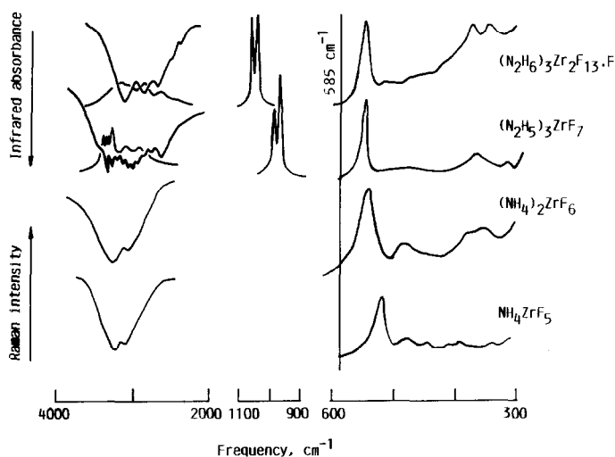
Fig. 2. Raman and IR spectra of (\text{N}_2\text{H}_5)_3\text{ZrF}_7 , compounds corresponding to its decomposition products, and (\text{N}_2\text{H}_6)_3\text{ZrF}_{13}\cdot\text{F} . 585\text{ cm}^{-1} : frequency of \nu_1 in octahedral \text{ZrF}_6^{2-} ions.
