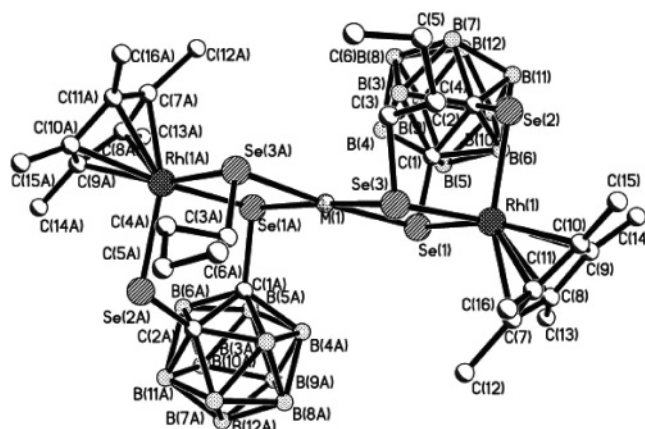
Figure 2. Molecular structures of 4 and 5 (30% probability). Hydrogen atoms are omitted for clarity. Selected distances (Å) and angles (deg) for 4 ( \text{M} = \text{Ni} ): Ni(1)–Se(1), 2.3727(11); Ni(1)–Se(3), 2.3119(11); Rh(1)–Se(3), 2.4459(10); Rh(1)–Se(1), 2.4562(9); Rh(1)–Se(2), 2.4643(11); Se(1)–C(1), 1.968(6); Se(2)–C(2), 1.924(7); Se(3)–C(13), 1.934(7); C(1)–C(2), 1.654(9); Se(3)–Ni(1)–Se(1), 85.04(3); Se(3)–Rh(1)–Se(1), 80.47(3); Se(3)–Rh(1)–Se(2), 94.26(3); Ni(1)–Se(1)–Rh(1), 96.10(4); Ni(1)–Se(3)–Rh(1), 97.99(4). Selected distances (Å) and angles (deg) for 5 ( \text{M} = \text{Pd} ): Pd(1)–Se(3), 2.4102(12); Pd(1)–Se(1), 2.4795(11); Rh(1)–Se(3), 2.4621(12); Rh(1)–Se(2), 2.4634(12); Rh(1)–Se(1), 2.4686(11); Se(1)–C(1), 1.955(7); Se(2)–C(2), 1.957(8); Se(3)–C(3), 1.918(8); C(1)–C(2), 1.627(9); Se(3)–Pd(1)–Se(1), 83.68(3); Se(3)–Rh(1)–Se(2), 94.28(4); Se(3)–Rh(1)–Se(1), 82.84(4); Se(2)–Rh(1)–Se(1), 91.57(4); Pd(1)–Se(1)–Rh(1), 95.63(4); Pd(1)–Se(3)–Rh(1), 97.61(5).
