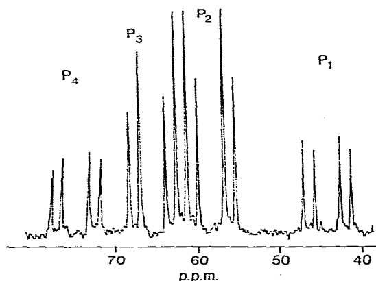
Fig. 5. ^{31}\text{P} NMR spectrum (obtained at 36.2 MHz) of the complex [\text{Rh}(\text{Cycphos})((Z)\text{-ethyl-}\alpha\text{-benzamido-cinnamate})]\text{PF}_6 in methanol shows the presence of two isomeric complexes.
