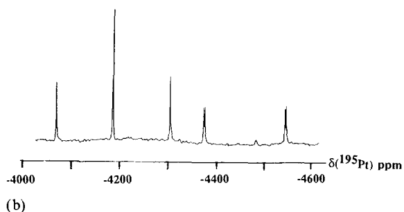
Fig. 1. NMR spectra of the solution obtained by mixing at -20^\circ\text{C} in dichloromethane equimolar quantities of \text{Pt}(\text{xan})_2 and dpm (spectra run at -20^\circ\text{C} ): (a) ^{31}\text{P} , (b) ^{195}\text{Pt} .
