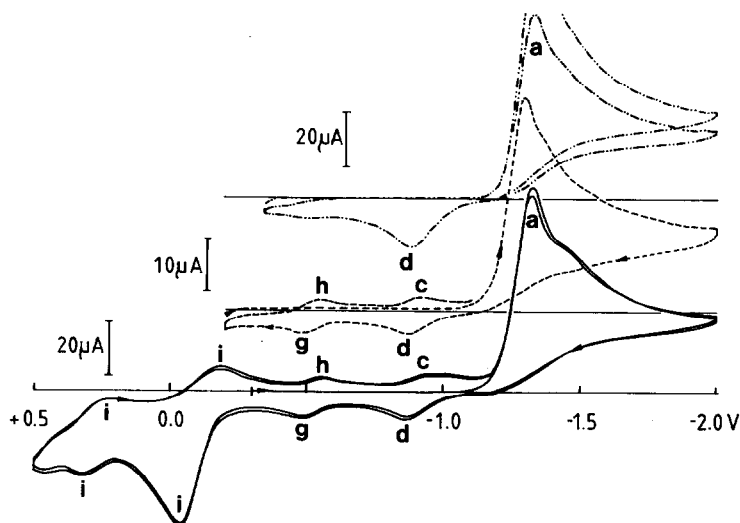
Fig. 2. Cyclic voltammogram of Ia ( 17.2 mg = 31 \mu\text{mol} ; 25^\circ\text{C} ; 0.1 M \text{Bu}_4\text{NClO}_4 in \text{CH}_3\text{CN} , 200 mV/s) —; repetition of a scan of Ia (arbitrary concentration) between -0.2 and -2 V to avoid the iodine depending redox waves i ( 100 mV/s); - - - - repetition ( 200 mV/s) in the presence of 240 \mu\text{mol} of \text{Bu}_4\text{NI} rel. to 31 \mu\text{mol} Ia - · - · - ·.
