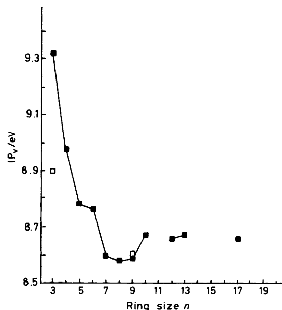
Figure 5. Plot of the experimental IP v s for series (2) (■) versus ring size. Experimental (□) IP v values for open-chain tosylalkylamines having the same number of carbon atoms are also shown
