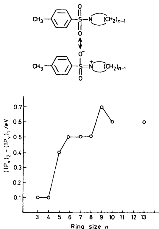
Figure 6. Difference in \text{IP}_v s between series (2) and (1) versus ring size
