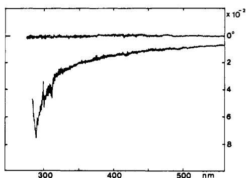
Figure 6. ORD curve of the alcohol derived from 3 and 24 taken at a concentration of 2.1 mg/0.1 mL of hexane.
