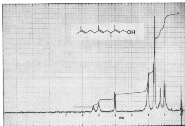
Figure 2. ^1\text{H} NMR spectrum (100 MHz) of a \text{CCl}_4 solution of the alcohol derived from the product ( 14 ) of the enzymatic reaction between 3 and 12 .
