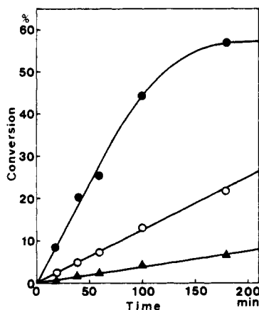
Figure 7. Time course of the conversion of isopentenyl pyrophosphate and its homologues into allylic products. The substrates were: (●) 1 and 2; (▲) 8 and 2; (○) 12 and 2.
