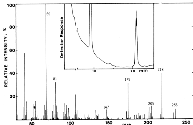
Figure 1. GLC-mass spectrum of the alcohol derived from the product ( 14 ) of the enzymatic reaction of 3 and 12 . The chromatography was carried out at a linear programmed temperature at a rate of 4 °C/min from 100 to 200 °C on a 1-m 5% poly(ethylene glycol) column with He gas at 25 mL/min. The inset shows the chromatogram. The perpendicular thin line on the peak indicates the position where the mass spectrum was measured.
